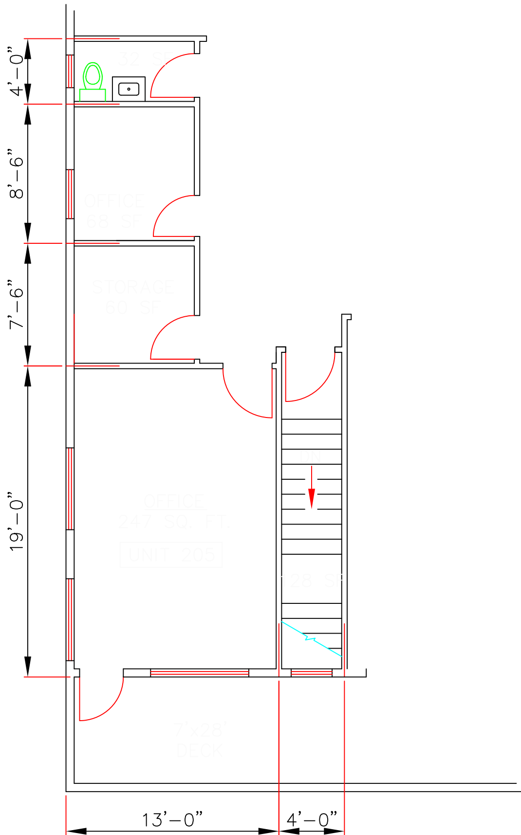
UNIT #205 FLOOR PLAN
