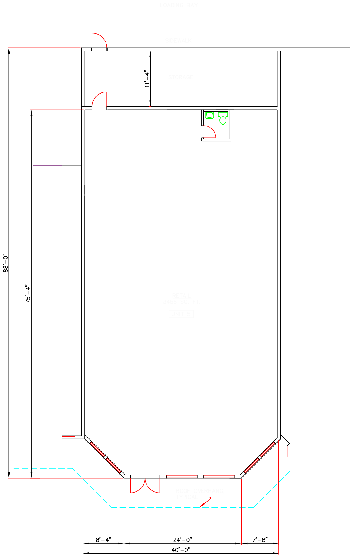
UNIT #5 FLOOR PLAN
